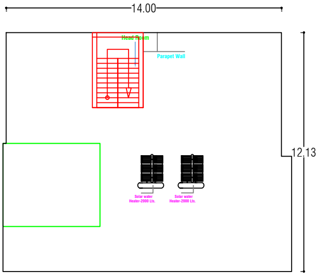
TERRACE PLAN & HEAD ROOM
