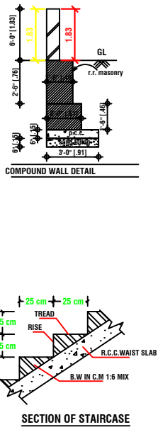
SECTION OF STAIRCASE
