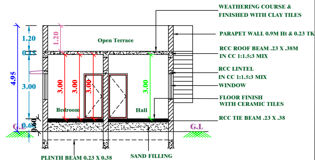
SECTION-XX
