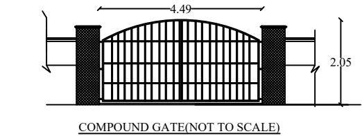
COMPOUND GATE(NOT TO SCALE)
