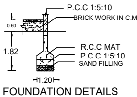
FOUNDATION DETAILS
