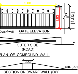
SECTION ON DWARF WALL (DW)
