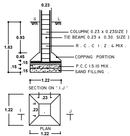
COLUMN FOUNDATION DETAIL'S ( NOT TO SCALE )
