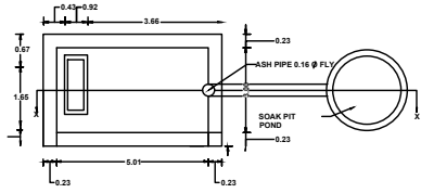
DETAIL OF SEPTIC TANK, [ SCALE 1:200 ]
