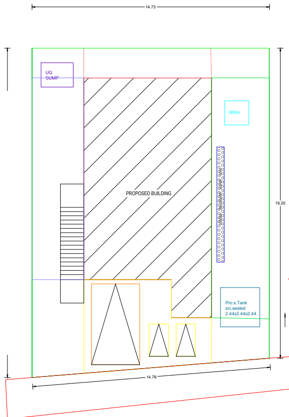
RAIN WATER HARVESTING SYSTEM RWH_CAPACITY_L=1000L/RS
