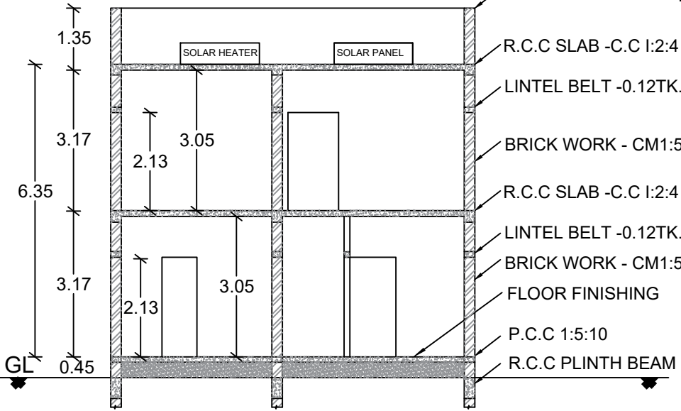
CROSS SECTION
