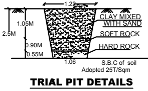
TRIAL PIT DETAILS
