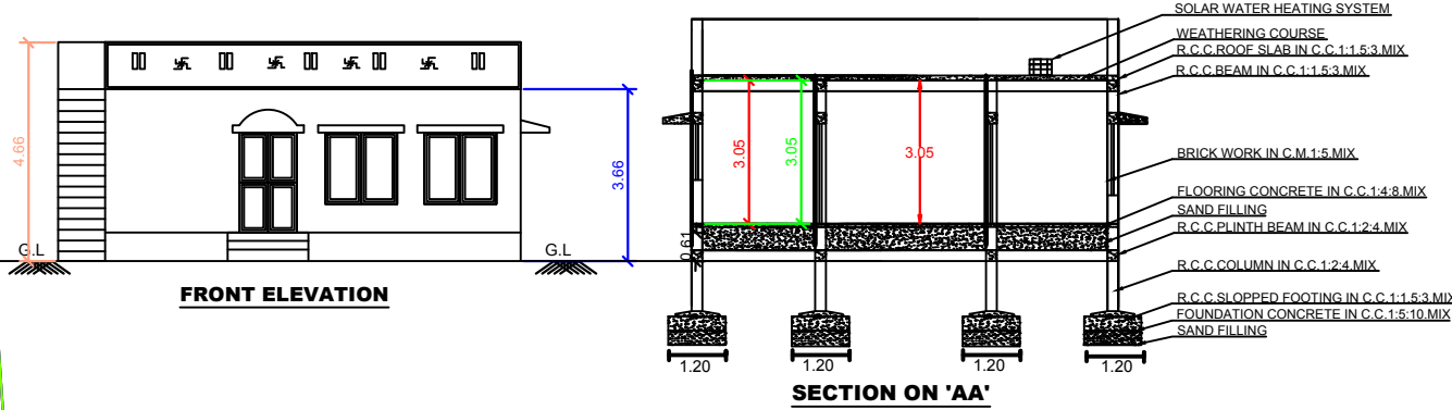
BORE WELL DETAIL
