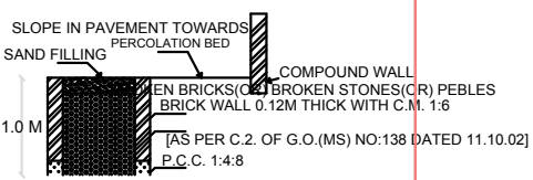
SECTION OF RAIN WATER PERCOLATION BED
