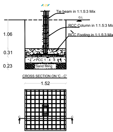
COLOUMN FOUNDATION
