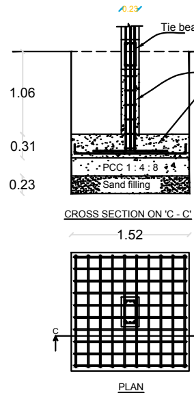
COLOUMN FOUNDATION
