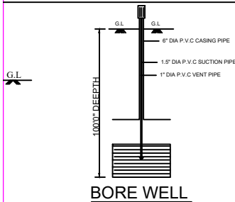
BORE WELL
