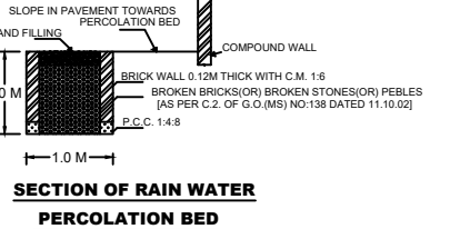
PERCOLATION BED
