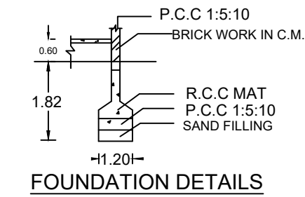
FOUNDATION DETAILS
