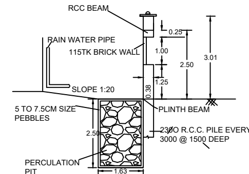
RAINWATER HARVESTING
