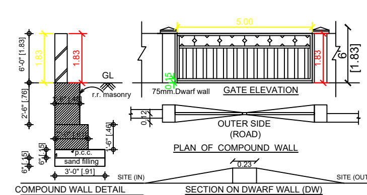
SECTION ON DWARF WALL (DW)
