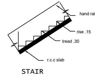
STAIR
