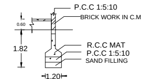
FOUNDATION DETAILS
