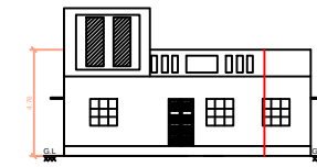
FRONT ELEVATION
