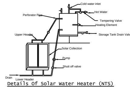
Details of Solar Water Heater (NTS)
