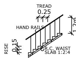
STAIRCASE DETAILS
