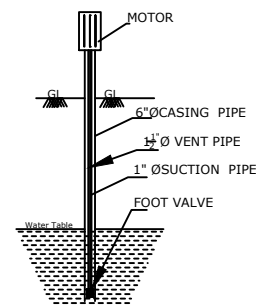
SEC. OF BOREWELL
