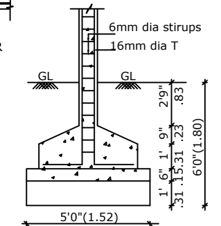
COLUMN FOUNDATION DETAIL
