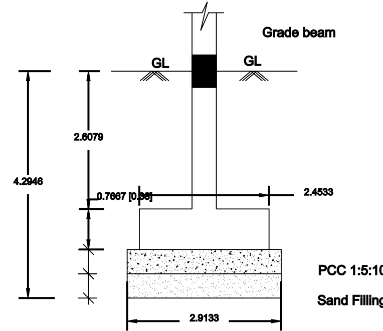
FOUNDATION DETAILS
