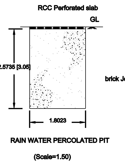
RAIN WATER PERCOLATED PIT (Scale=1.50)
