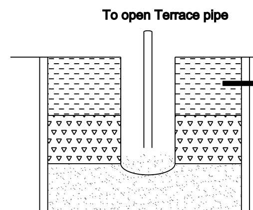
RAIN WATER COLLECTION CHAMBER
