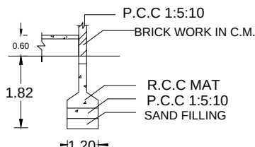
FOUNDATION DETAILS
