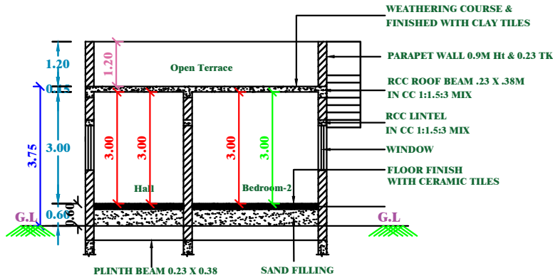
SECTION X-X
