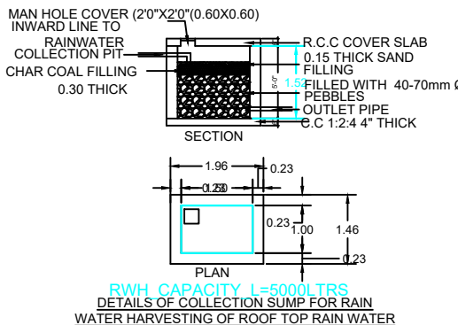
RAINWATER HARVESTING
