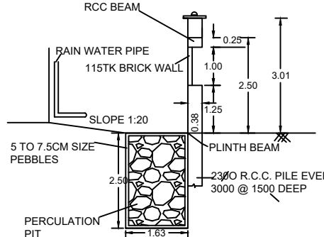
RAINWATER HARVESTING
