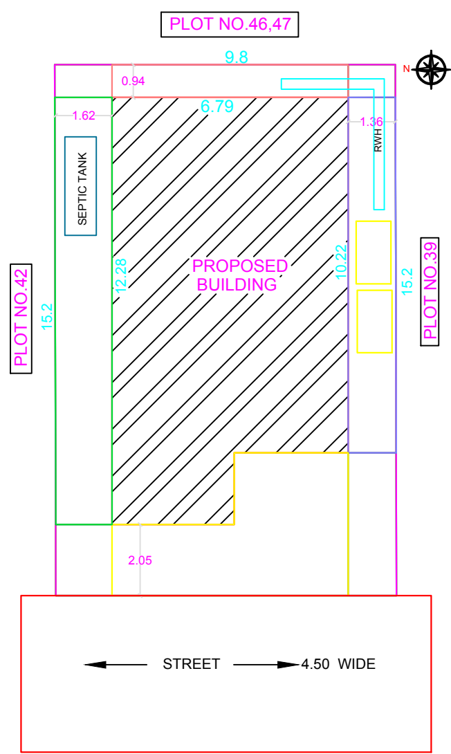
SITE PLAN
