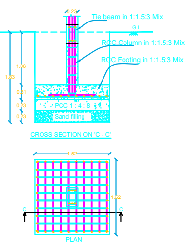
COLOUMN FOUNDATION DETAILS
