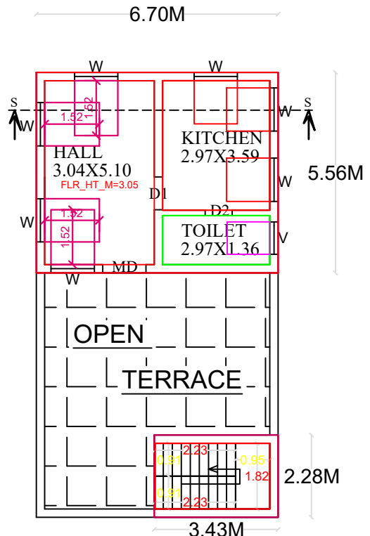
PROPOSED FIRST FLOOR
