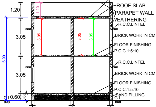
SECTION ON SS
