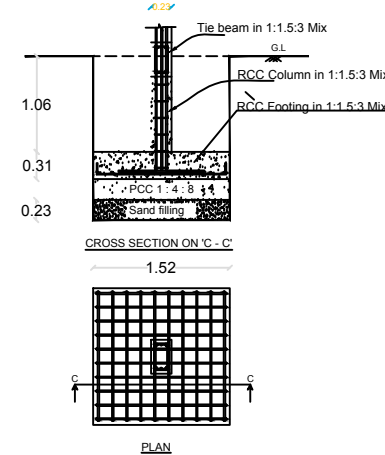
COLOUMN FOUNDATION
