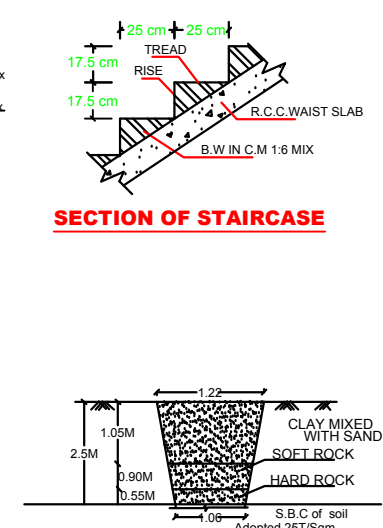
TRIAL PIT DETAILS
