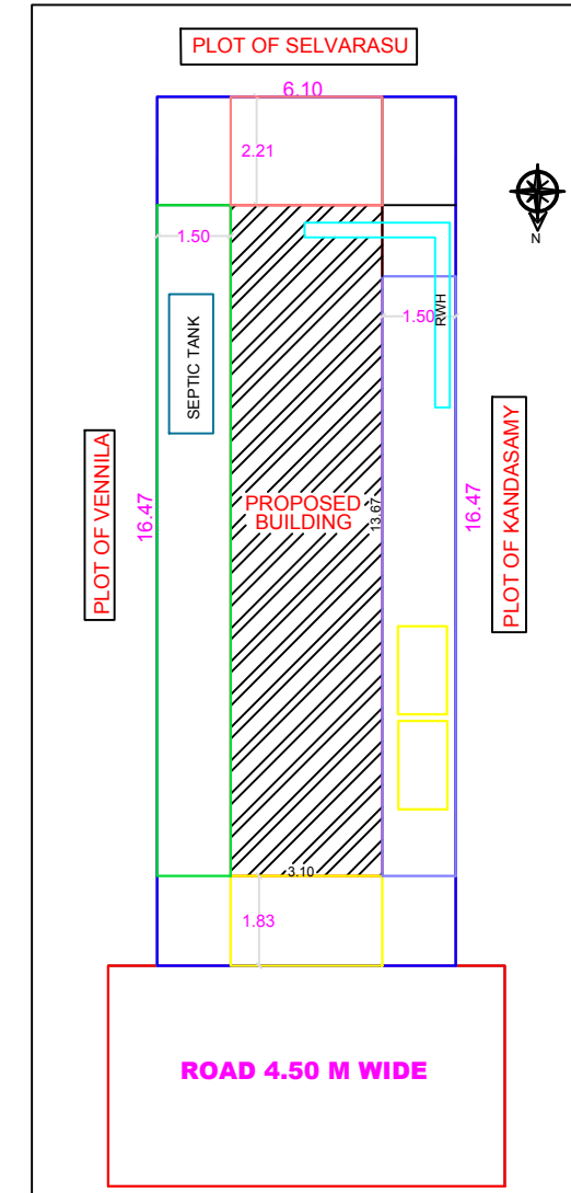
SITE PLAN
