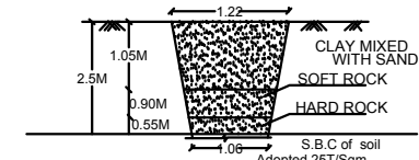
TRIAL PIT DETAILS
