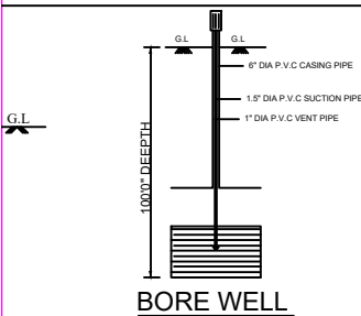
BORE WELL
