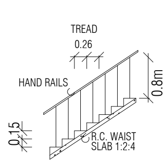
STAIRCASE DETAILS
