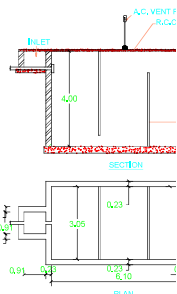
PLAN & SECTION OF SEPTIC TANK & DISPERSION TRENCH
