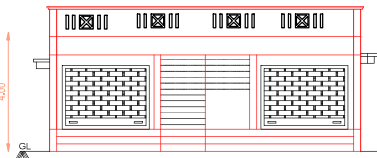
FRONT ELEVATION
