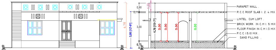
FRONT ELEVATION
