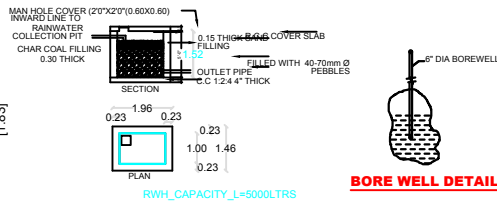
DETAILS OF RAINWATER HARVESTING
