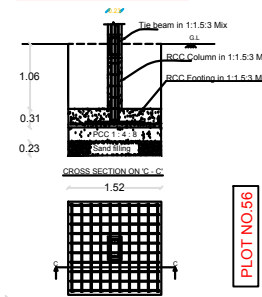
COLOUMN FOUNDATION
