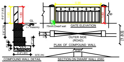
DETAILS OF COMPOUND WALL
