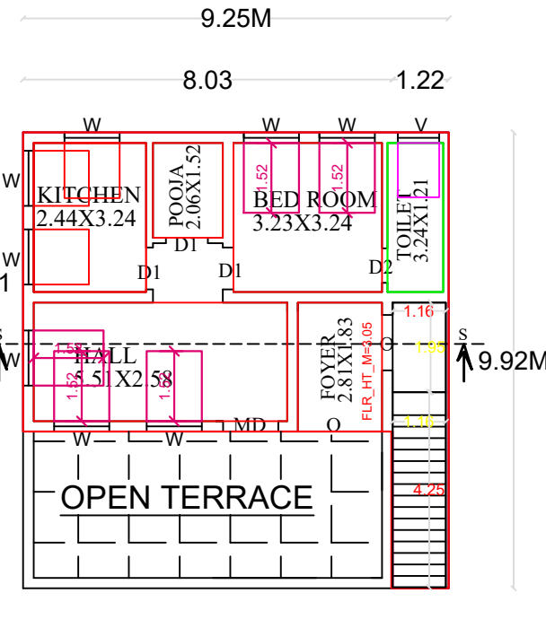
PROPOSED FIRST FLOOR
