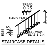
STAIRCASE DETAILS
