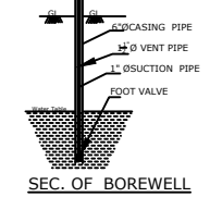
SEC. OF BOREWELL
