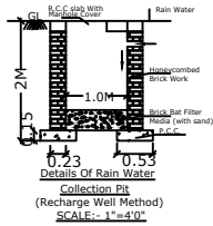
SEC. OF RAIN WATER COLLECTION PIT (Recharge Well Method) SCALE:- 1"=4'0"
