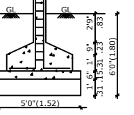
COLUMN FOUNDATION DETAIL
