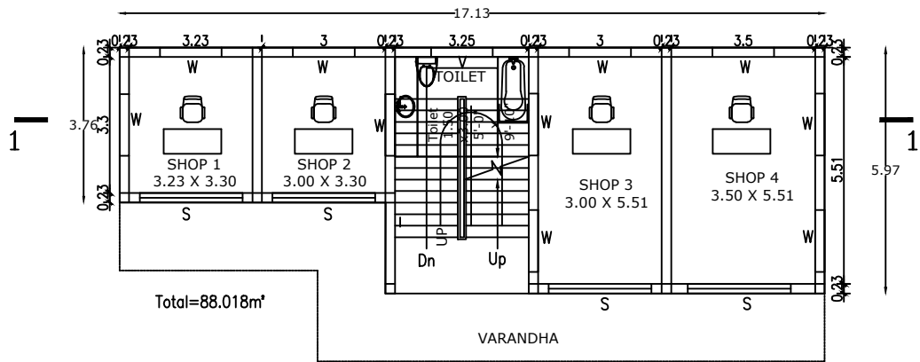
PRO. GROUND FLOOR PLAN
