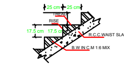
SECTION OF STAIRCASE
