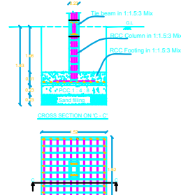
COLOUMN FOUNDATION DETAILS
