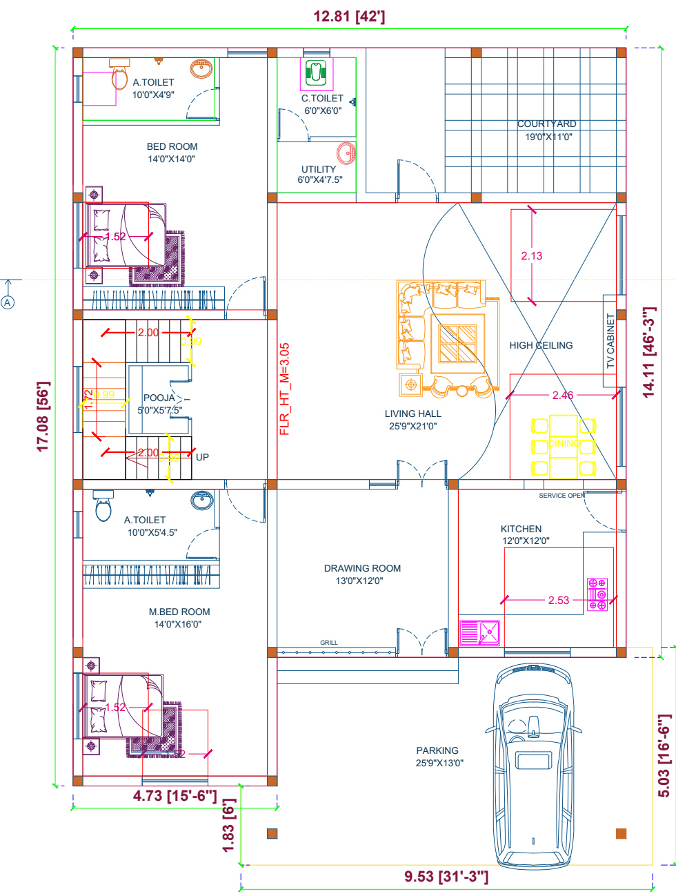
PROPOSED GROUND FLOOR PLAN ( SOUTH FACING )
