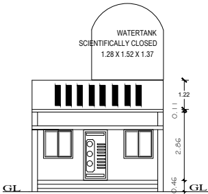
FRONT ELEVATION NORTH FACING.
