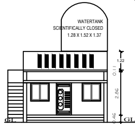
FRONT ELEVATION SOUTH FACING.
