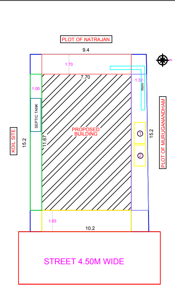
SITE PLAN
