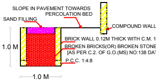
SECTION OF RAIN WATER PERCOLATION BED
