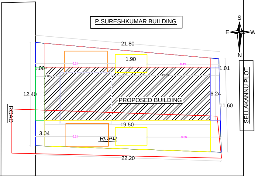
SITE PLAN : [1:100] SCALE
