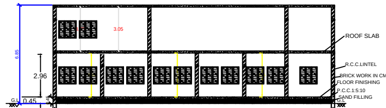
SECTION ON SS
