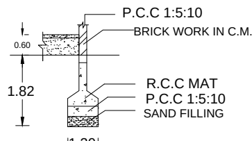
FOUNDATION DETAILS
