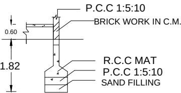
FOUNDATION DETAILS
