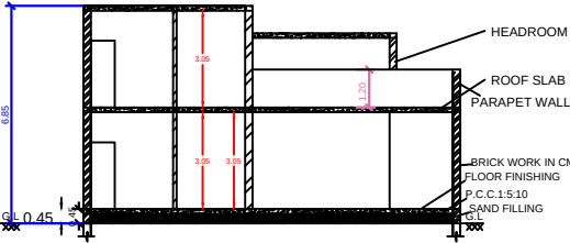
SECTION ON XX
