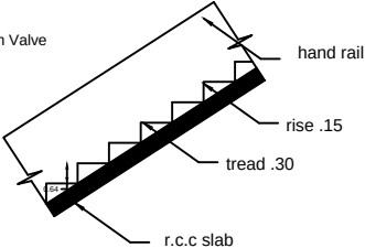
STAIR
