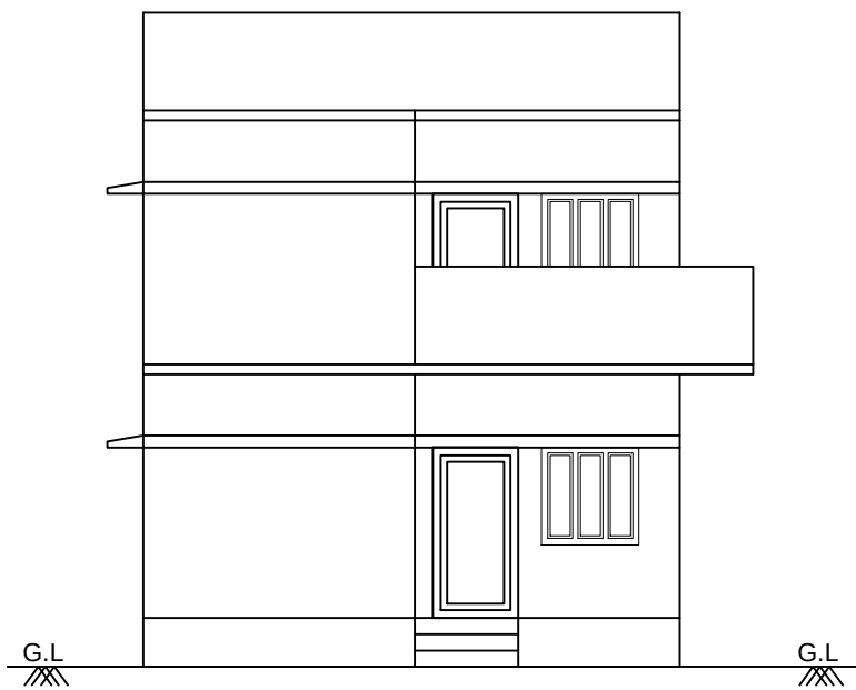
FRONT ELEVATION
