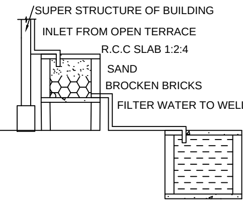
RAINWATER HARVESTING
