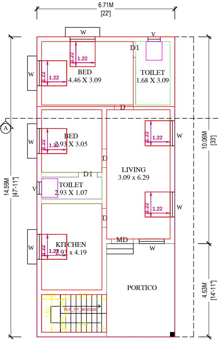
EX. AND PRO.GOUND FLOOR PLAN
