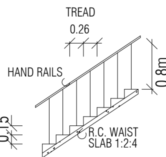
STAIRCASE DETAILS
