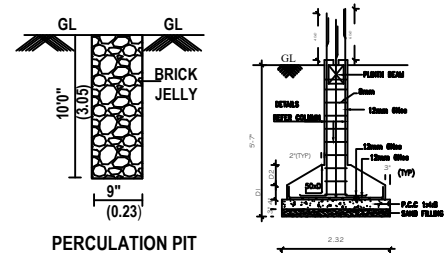
FOUNDATION DETAILS SCALE : 1:50.
