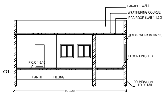
SECTION "A-B"
