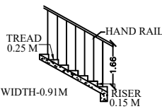
STAIRCASE DETAILS
