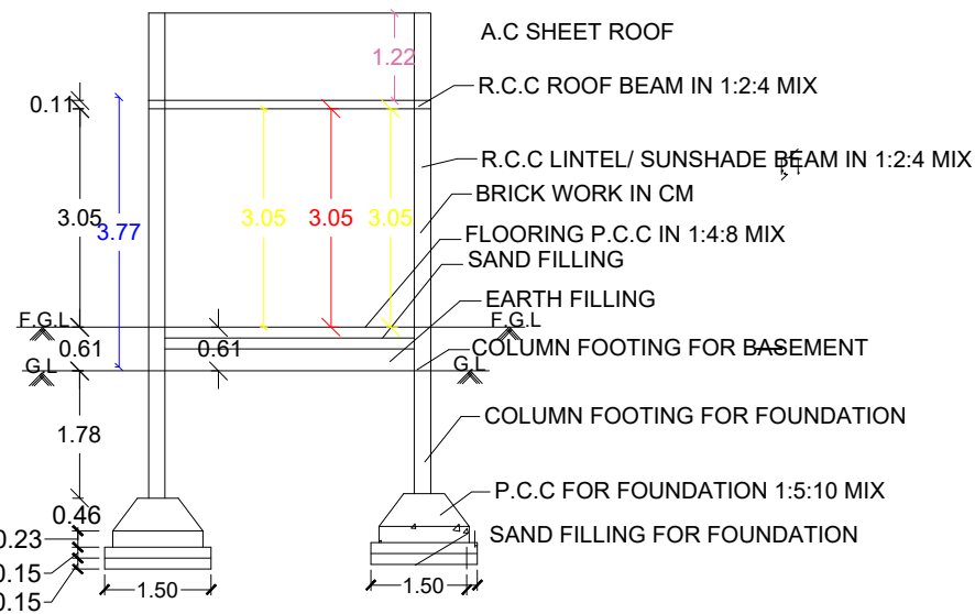
SECTION ON-AA
