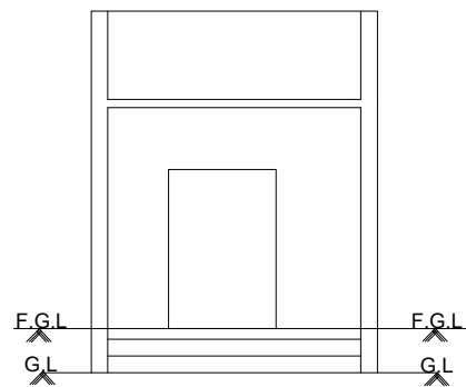
FRONT ELEVATION SOUTH FACING
