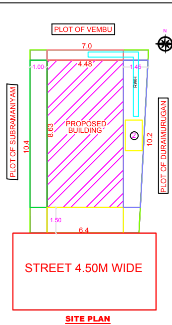
SITE PLAN
