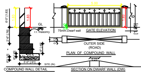
DETAILS OF COMPOUND WALL
