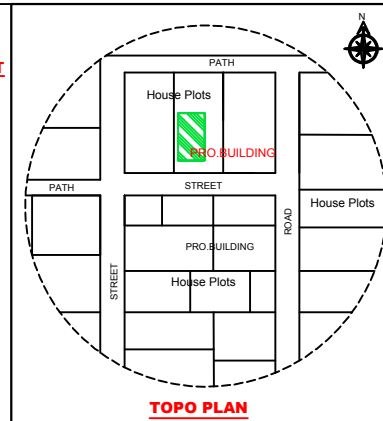
TOPO PLAN
