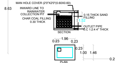
DETAILS OF RAINWATER HARVESTING
