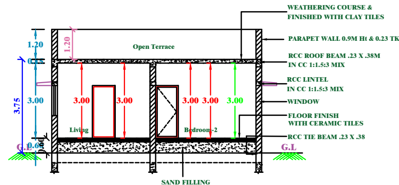
SECTION-XX
