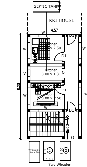
SITE CUM PRO. GROUND FLOOR PLAN
