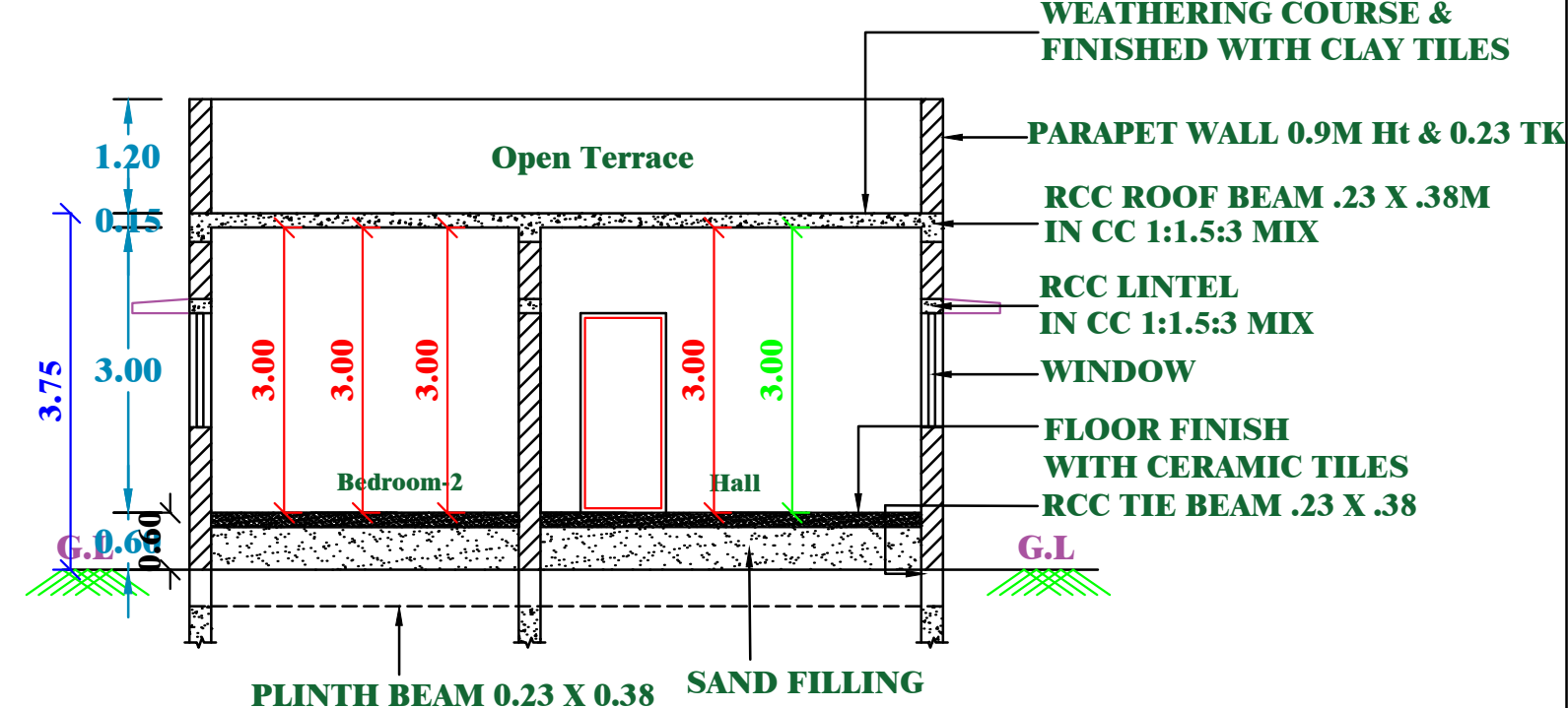
SECTION-'X-X'
