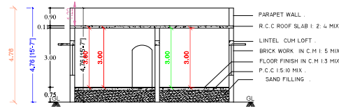
CROSS SECTION ON 'AB'
