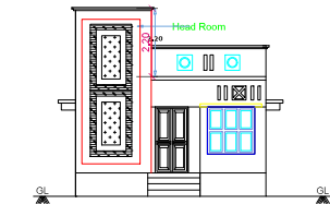
FRONT ELEVATION
