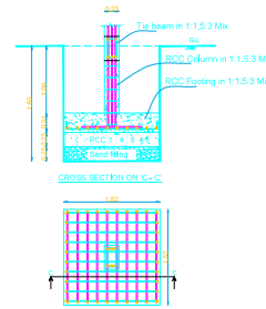
COLOUMN FOUNDATION DETAILS - A
