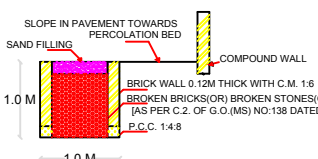
SECTION OF RAIN WATER PERCOLATION BED
