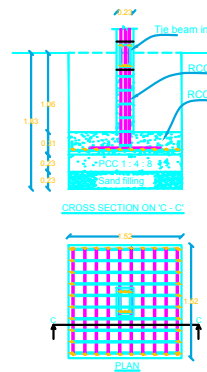
COLOUMN FOUNDATION DETAILS
