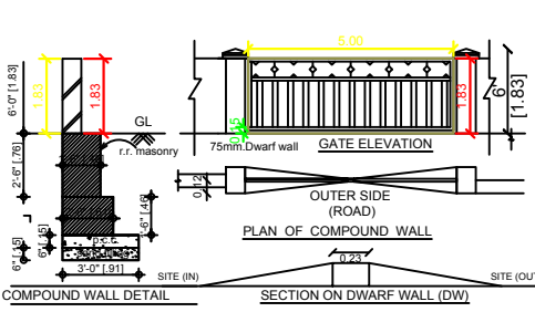
DETAILS OF COMPOUND WALL
