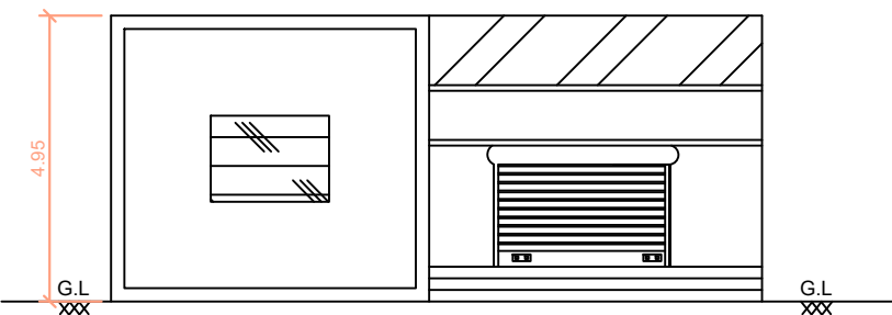
FRONT ELEVATION
