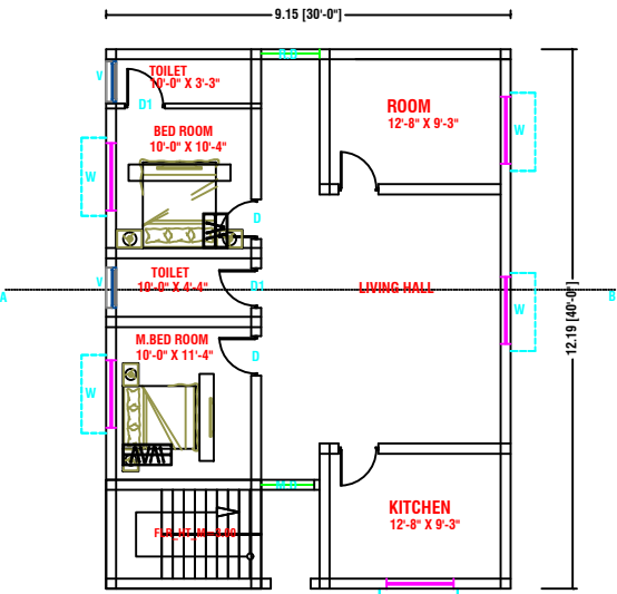
GROUND FLOOR PLAN (SOUTH FACING)
