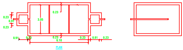
PLAN & SECTION OF SEPTIC TANK & DISPERSION TRENCH
