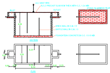
PLAN & SECTION OF SEPTIC TANK & DISPERSION TRENCH
